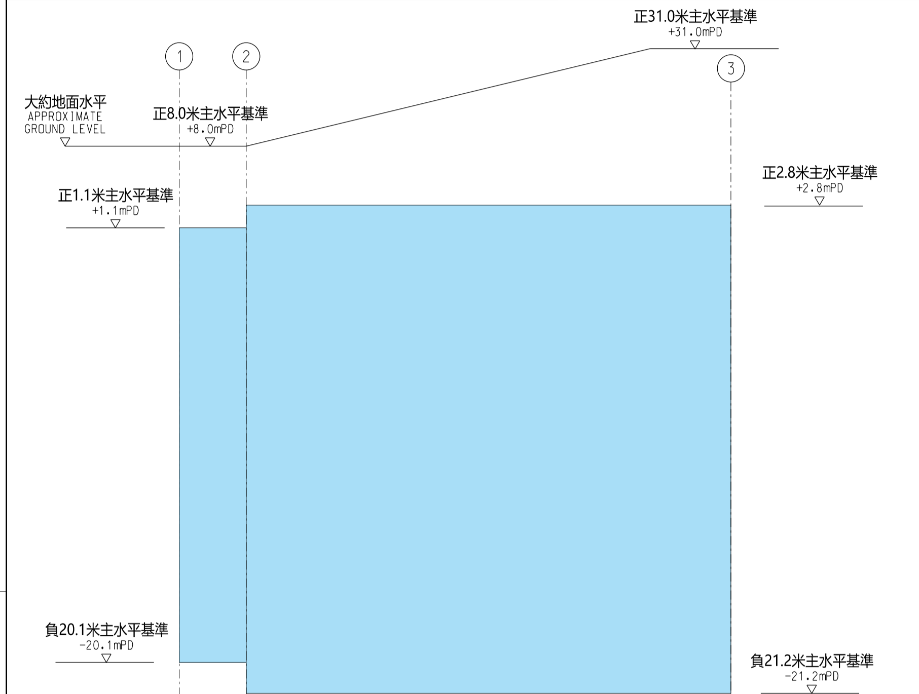
沿參線的 切面立視圖 SECTIONAL ELEVATION ALONG REFERENCE LINE 不按比例 NOT TO SCALE
